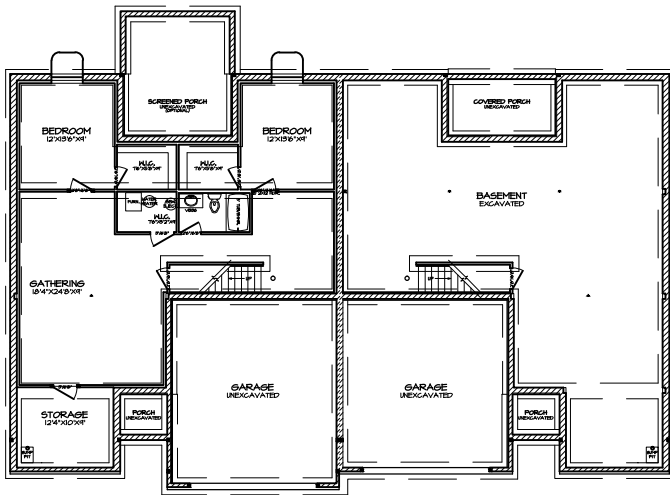
FOUNDATION PLAN A-1
