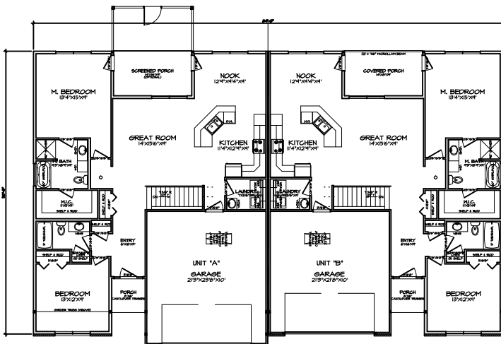
FIRST FLOOR PLAN A-1
